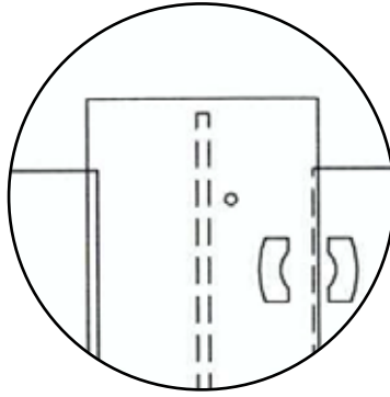
Front View of the Middle Pilaster showing the Hinge Fixing
